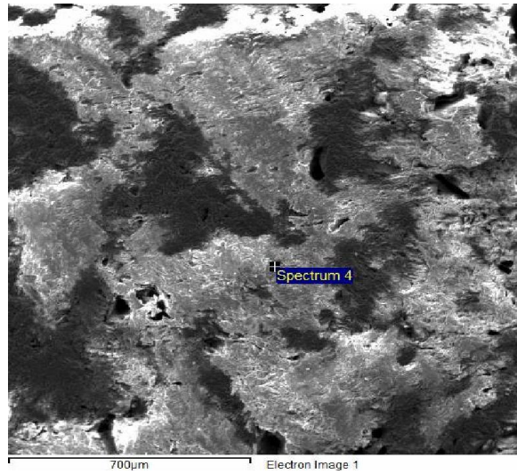
Fig. 12. SEM image of marble onyx, sample 4
