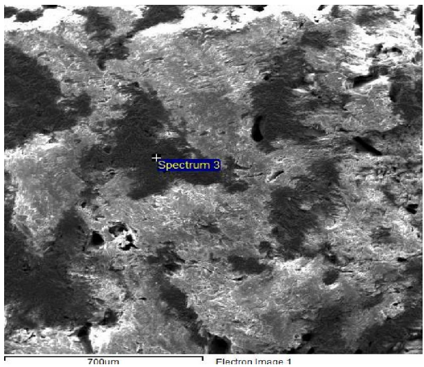
Fig. 11. SEM image of marble onyx, sample 3
