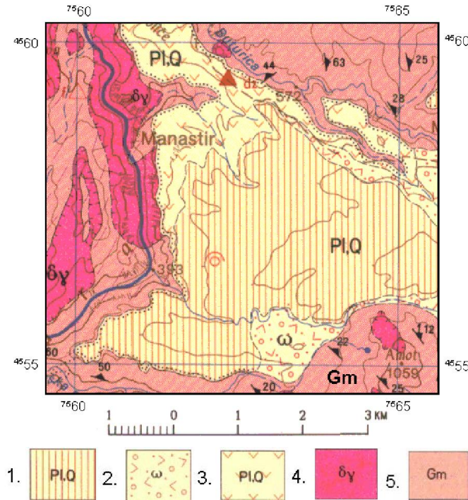
Fig. 2. Geological map of the locality of Bešište village BGM SFRY 1:100 000, sheet Vitolište. 1 – travertine and onyx, 2 – carbonate-tuffaceous products, 3 – volcanic sediment products, 4 – granodiorite, 5 – gneisses
