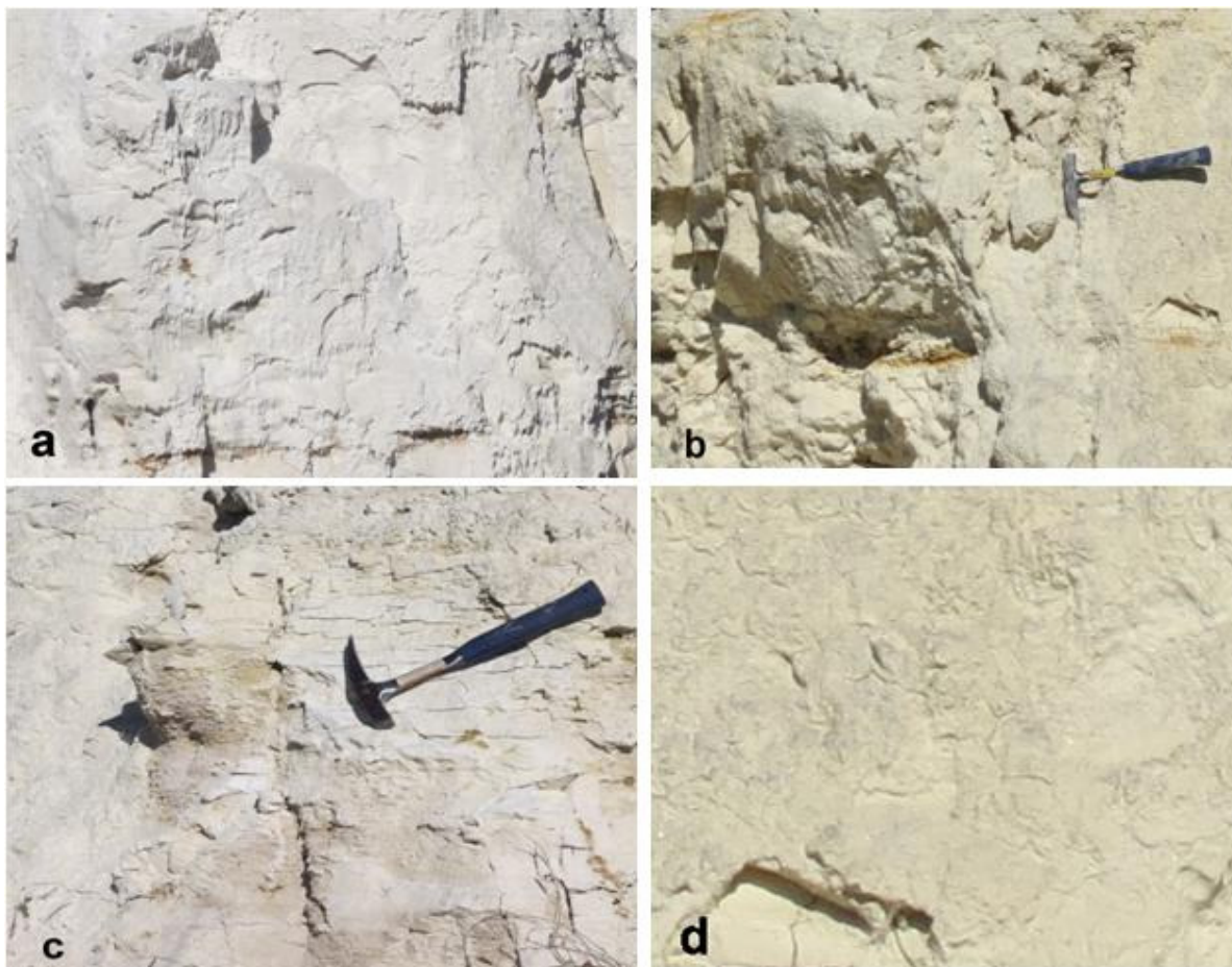
Fig 6. The most common types of diatomaceous earth a) Grey ashy diatomaceous earth with plated habitus. b) White diatomaceous earth with shelly defraction. c) White sheeted diatomaceous earth. d) Yellow diatomaceous earth
