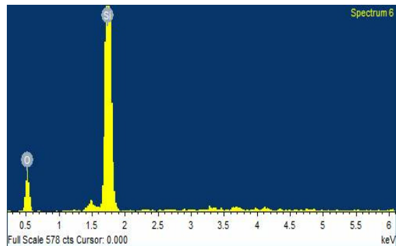
Fig. 19. EDC spectrum of diatomaceous earth, sample 6
