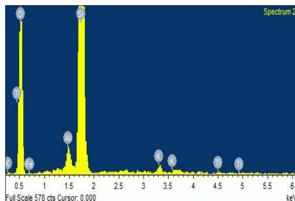
Fig. 11. EDC spectrum of diatomaceous earth, sample 2
