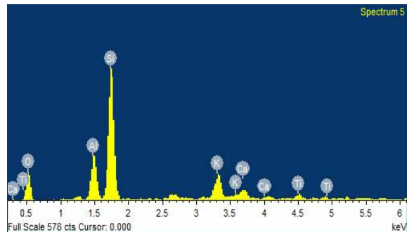
Fig. 18. EDC spectrum of diatomaceous earth, sample 5
