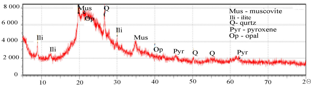
Fig. 7. X-ray diffractogram of diatomaceous earth from the Manastir-Bešište deposit
