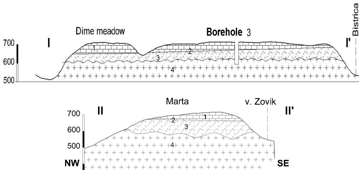
Fig. 3. Characteristic geological profiles
