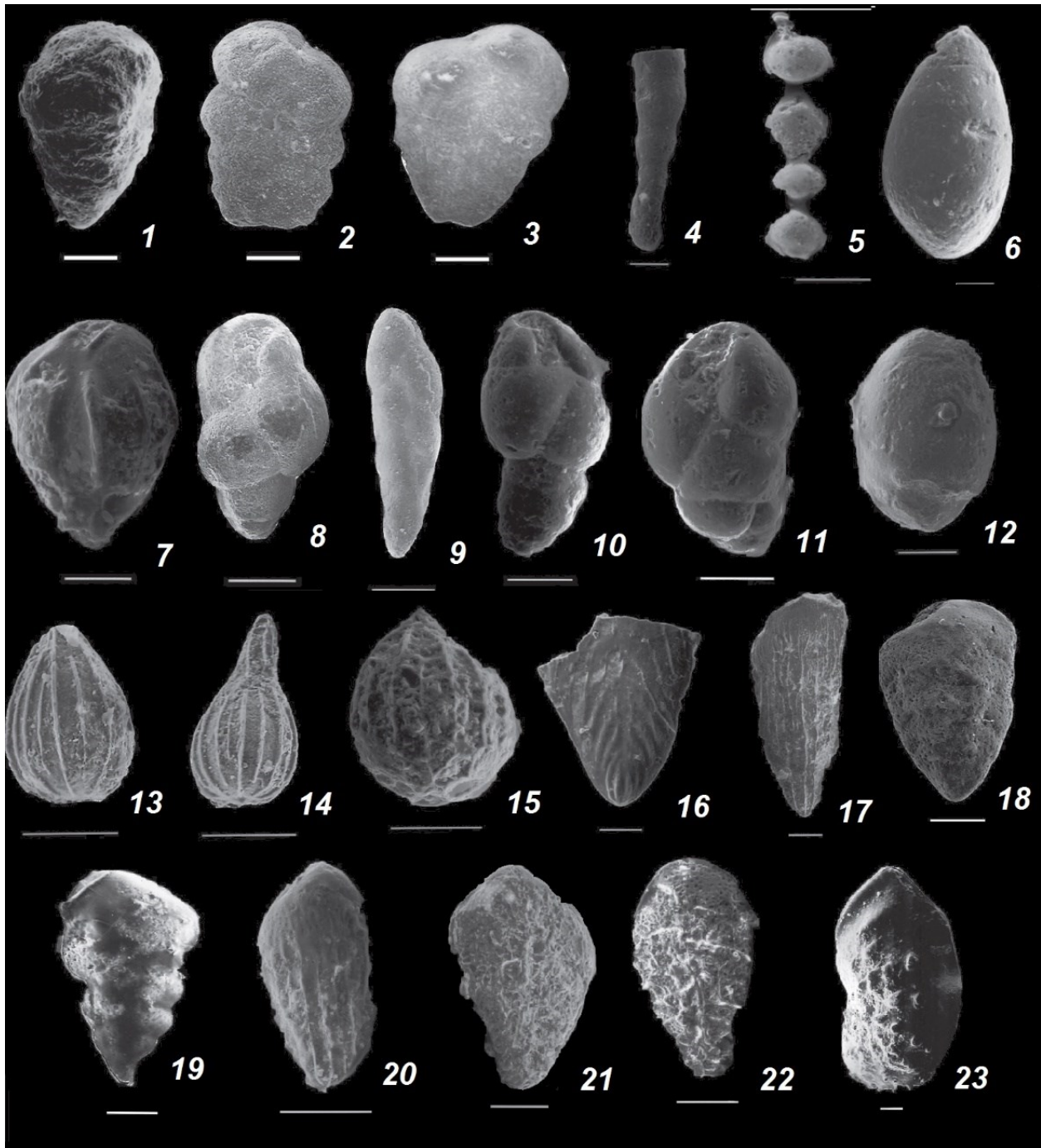
PLATE II: Tapered and cylindrical morphogroup (T/C): 1. Marssonella indentanta (Cushman et Jarvis): Nemanjici section, SEM×200. 2. Textularia bronniata (d'Orbigny): Čardaklija section, SEM×156. 3. Textularia minuta Terquem: Čardaklija section, SEM×178. 4. Nodosaria sp.: Nemanjici section, SEM×200. 5. Siphonodosaria adolphina (d'Orbigny): Nemanjici section, SEM×110. 6. Glandulina ovula d'Orbigny: Nemanjici section, SEM×400. 7. Bulimina sculptilis Cushman: Nemanjici section, SEM×300. 8. Bulimina trigona Terquem: Čardaklija section, SEM×186. 9. Fursenkoina dibollensis (Cushman et Applin): Čardaklija section, SEM×101. 10. Caucasina eocenica Chalilov: Nemanjici section, SEM×240. 11. Caucasina tenebricosa Pishvanova: Nemanjici section, SEM×300. 12. Chilostomelloides balkhanensis (Dain et Chalilov): Nemanjici section, SEM×250. Spherical morphogroup (S): 13. Lagena humifera Bandy: Čardaklija section, SEM×221. 14. Lagena striata (d'Orbigny): Čardaklija section, SEM×221. 15. Favulina hexagona (Williamson): Nemanjici section, SEM×340. Flattened tapered morphogroup (FT): 16. Palmula budensis (Hantken): Nemanjici section, SEM×180. 17. Bolivina cf. antegressa Subbotina: Nemanjici section, SEM×140. 18. Bolivina cf. cookei Cushman, 1922: Nemanjici section, SEM×250. 19. Bolivina gracilis Cushman and Applin: Nemanjici section, SEM×185. 20. Bolivina nobilis Hantken: Nemanjici section, SEM×325. 21. Bolivina reticulata Hantken: Nemanjici section, SEM×250. 22. Bolivina scalprata Schwager: Nemanjici section, SEM×250. Heteromorphous morphogroup (H): 23. Percultazonaria fragaria (Gümbel): Nemanjici section, SEM×110.
