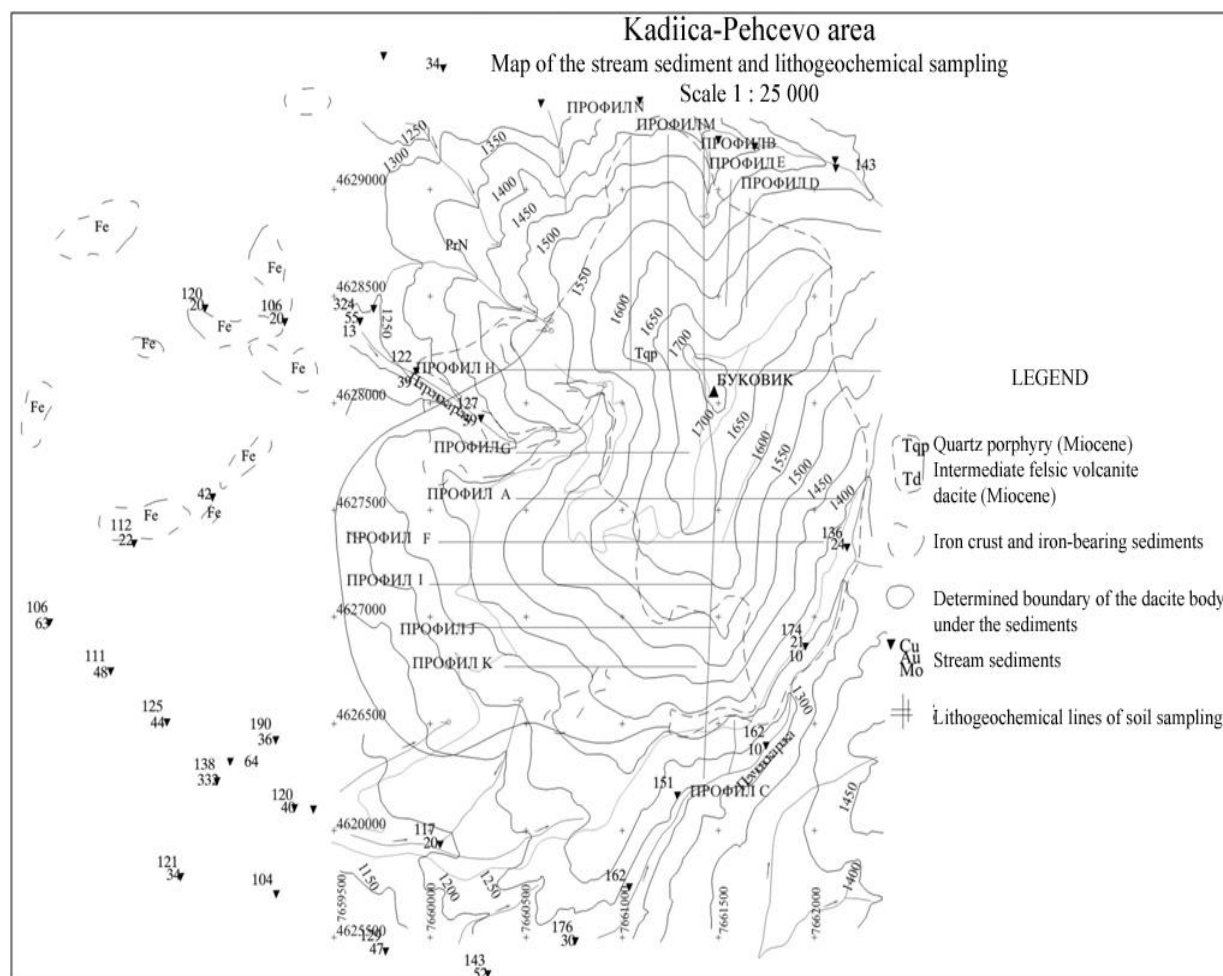
Fig. 4. Map of the lithochemical sampling and stream sediments (Aleksandrov and Bombol., 2007)
