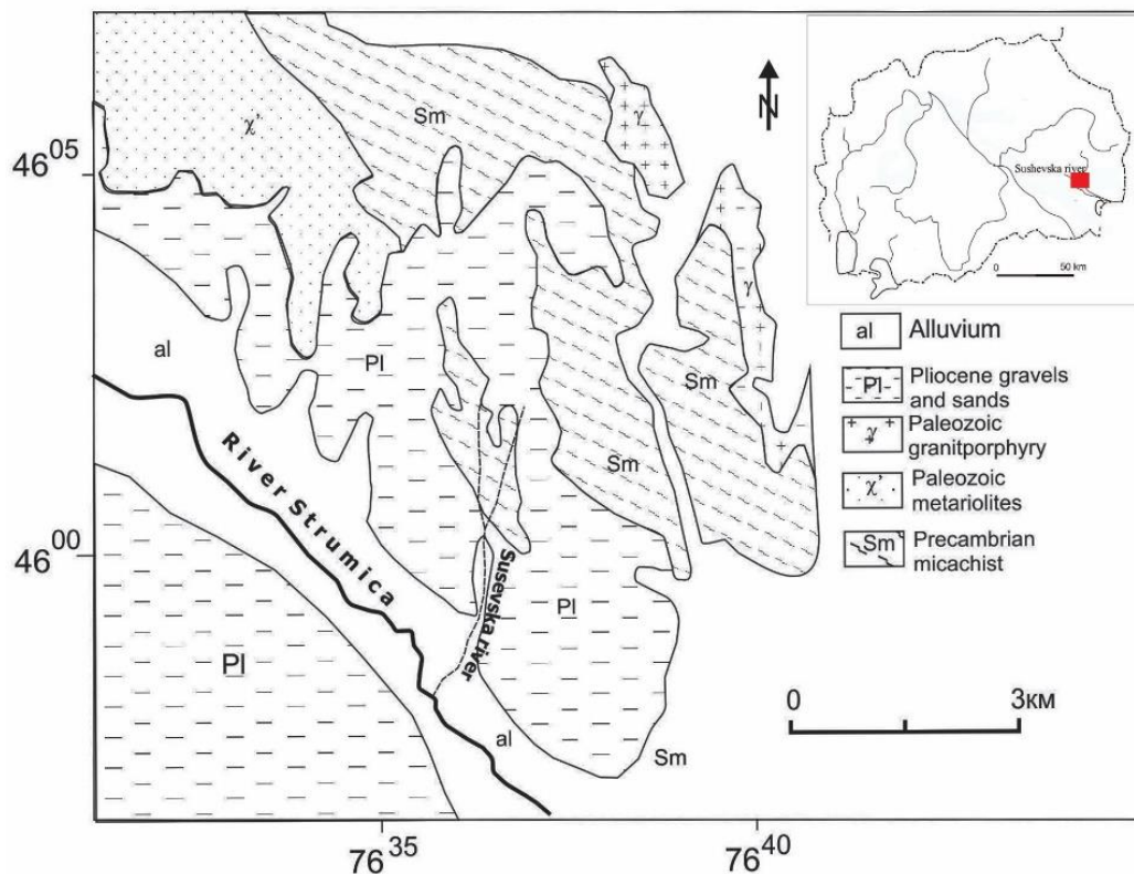
Fig. 1. Simplified geological map at study area
