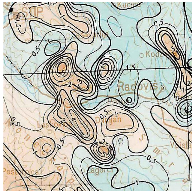
Fig. 4. Part of the Map of the vertical geomagnetic Z-component of the Lakavica depression (Map of the Vertical Z-component 1 : 500 000)
