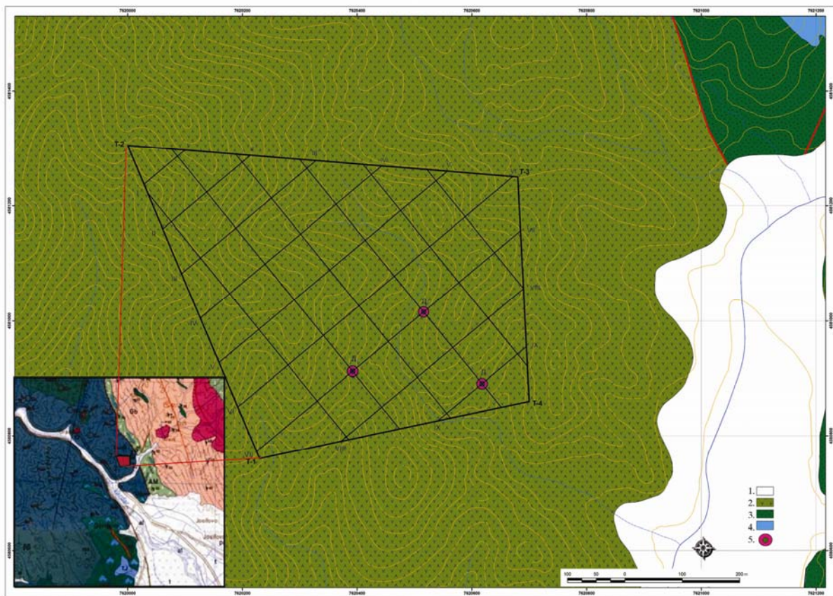
Fig. 1. Geological map of the locality Udovo (Спасовски и др., 2010) 1. alluvial sediments, 2. diabase, 3. amphibolite schists, 4. marbles, 5. drill hole
