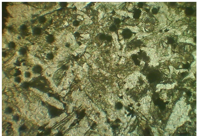
Fig. 6. Uniting the amphibole, pyroxene and plagioclase in subophitic structure ( N^- )
