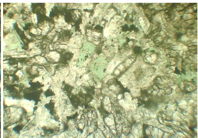
Fig. 8. Ophitic-subophitic structure of diabase consisted of barred and rectangular plagioclase whose gap is filled with pyroxene – augite ( N^- )
