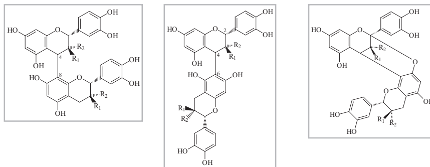
C4-C8 врска C4-C8 bond
