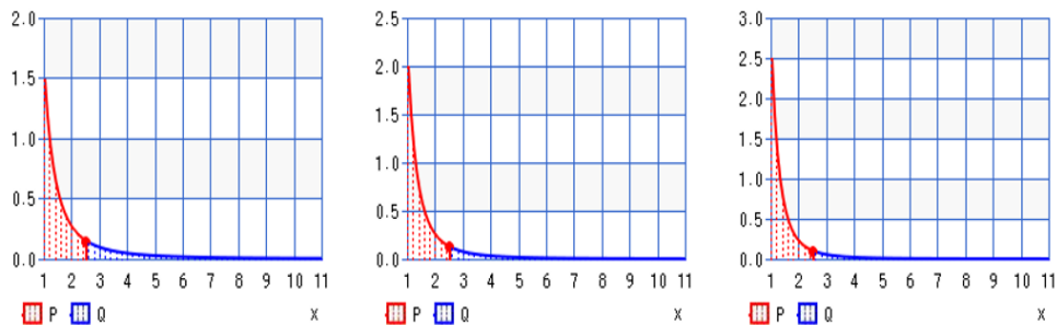
Figure 1 Pareto distribution function with shape parameter \alpha \in (1.5, 2, 2.5)
